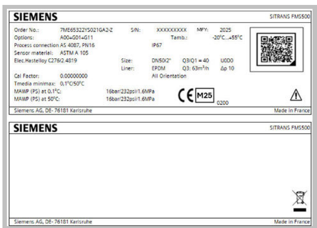
Sensor label
