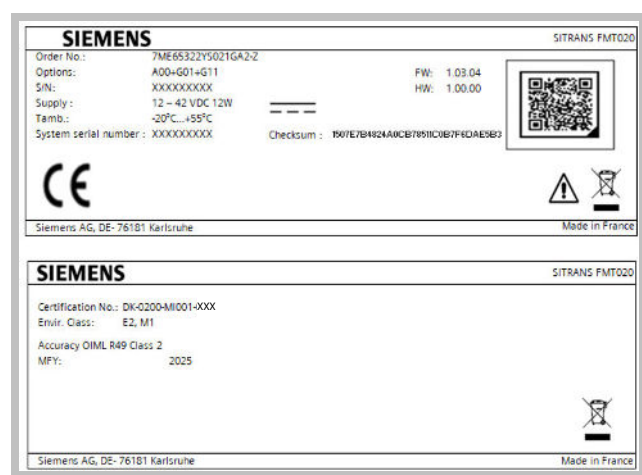
Transmitter label
