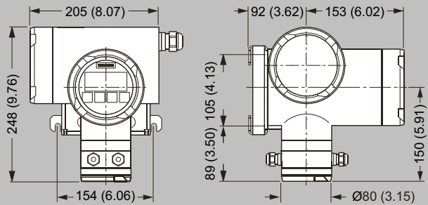
SITRANS FM transmitter TRANSMAG 2 with special wall-mounting bracket, dimensions in mm (inch)
