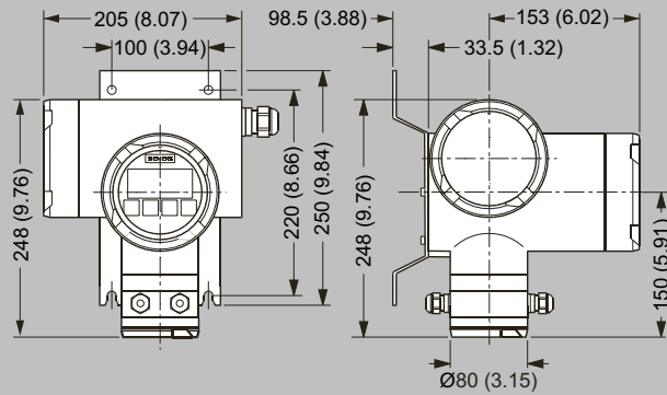
SITRANS FM transmitter TRANSMAG 2 with wall-mounting bracket, dimensions in mm (inch)
