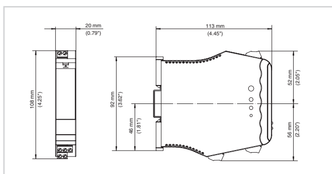
Dimensions VEGATRENN 141
