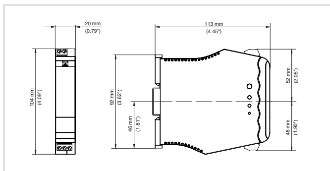
Dimensions VEGATRENN 151
