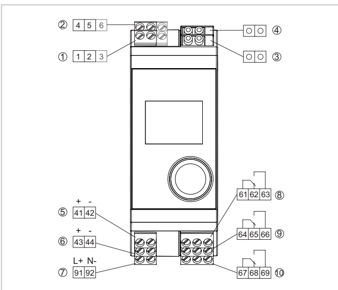
Wiring plan VEGAMET 142
