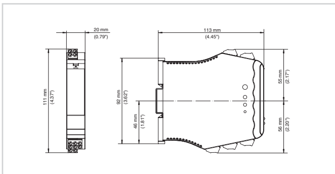
Dimensions VEGATOR 122
