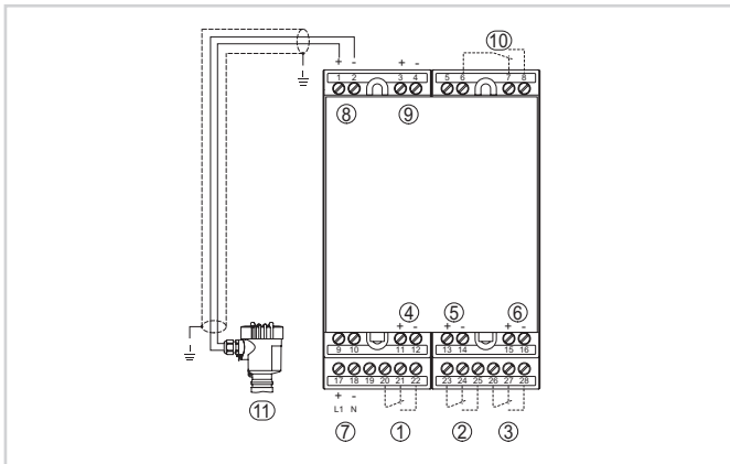
Connection VEGAMET 624 with two-wire sensor
