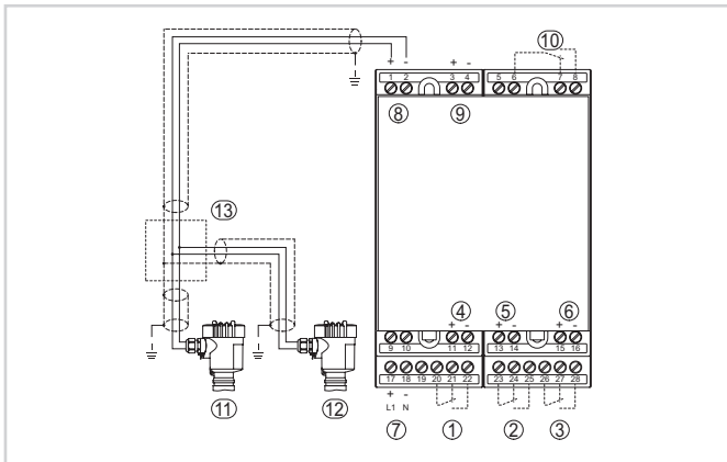
Connection VEGAMET 625 with two-wire sensors
