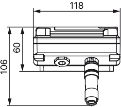
Compact variant with connector
