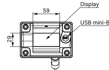
Compact variant with cable gland
