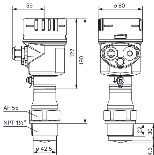
Variant NPT 1 1/2" PN 3 (ASME B1.20.1)
