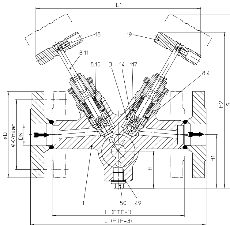
Stop valve with gland packing (inlet-right)
