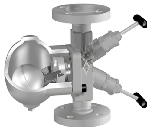
CONA®SC All-in-one (shown with optional drain plug)
