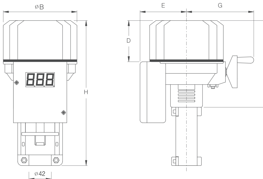
GEA-20PD, 35PD
