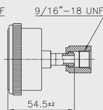
Swivel female
