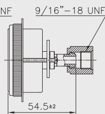
Swivel female
