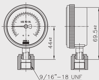
Swivel female
