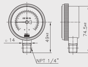
NPT male
