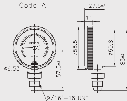
Swivel male
