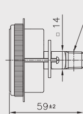
NPT male
