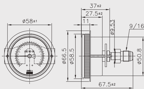
Swivel male
