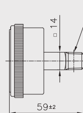
NPT male
