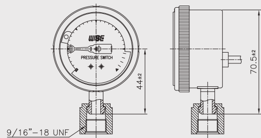
Swivel female
