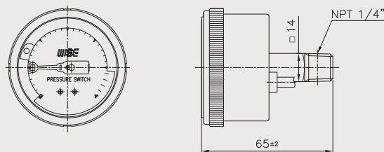
NPT male
