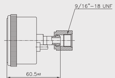
Swivel female
