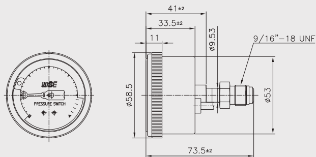
Swivel male
