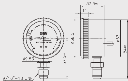
Swivel male
