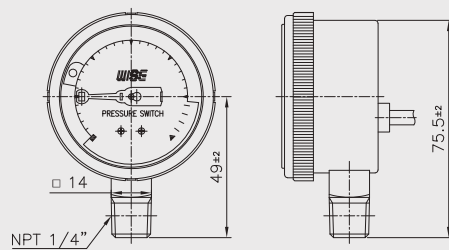
NPT male
