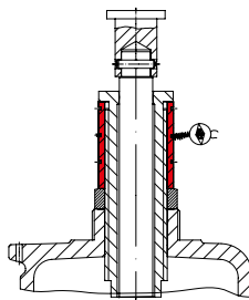
Lock bush
