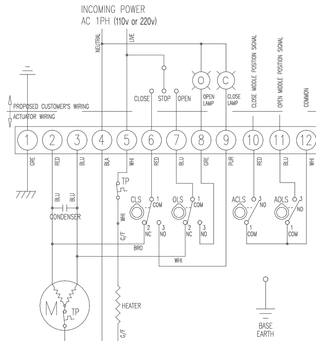
ON-OFF wiring GQ-010A [110 or 220VAC, 50/60Hz]
