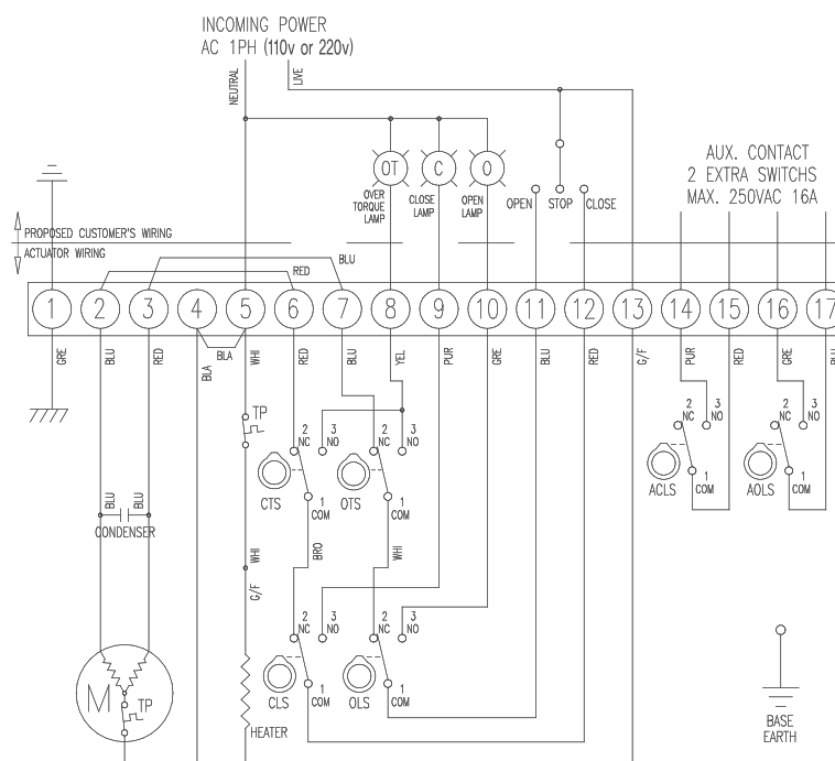
ON-OFF wiring GQ-016A ~ 300A [110 or 220VAC, 50/60Hz]
