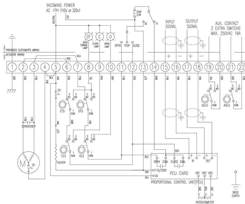
Proportional wiring GQ-016P ~ 300P [110 or 220VAC, 50 / 60Hz] - PCU
