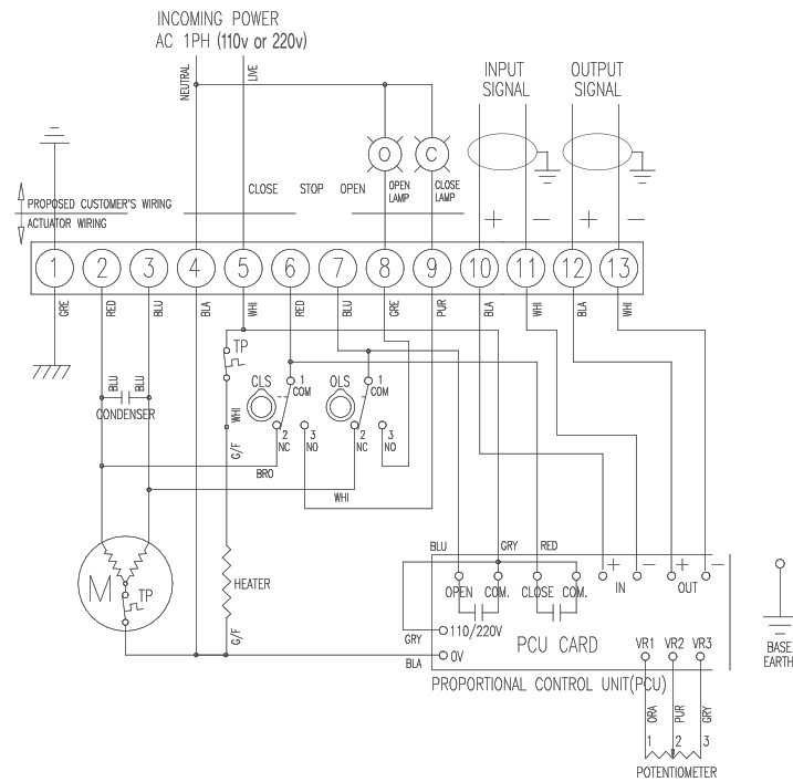
Proportional wiring GQ-010P [110 or 220VAC, 50 / 60Hz] - PCU
