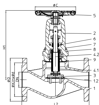
Fig. 141....153 DN15-150 / NPS 1/2"-6" One-piece stem
