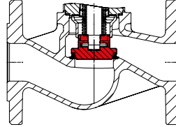
Plug with soft seal Max. operating temperature 200°C at PTFE + 25% carbon
