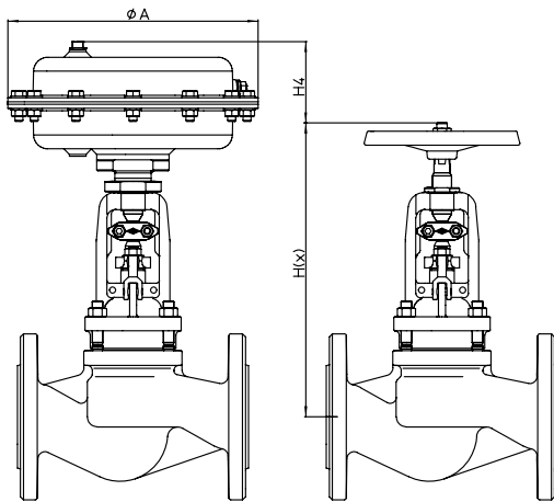
Spring closes (Extended stem on air failure)
