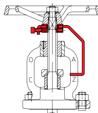
Position indicator with locking device
