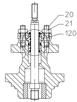
I. EPDM-sealing
