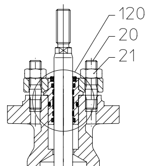
I. EPDM-sealing
