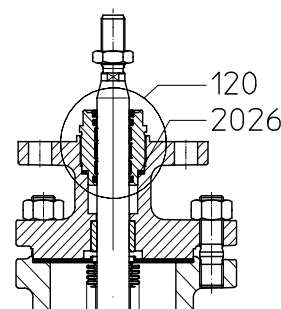
III. Stainless steel bellows seal with EPDM-sealing
